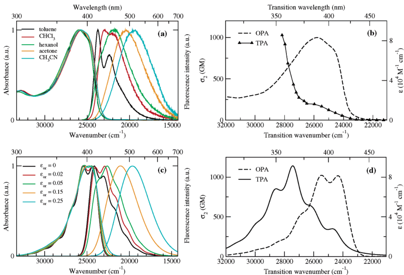
Figure 5. Spectra of compound 1 . (Left panels) Experimental (a) and calculated (c) absorption and fluorescence spectra in solvents of increasing polarity. (Right panels) Experimental (b) and calculated (d) OPA and TPA spectra of 1 in toluene. 1 GM = 10 -50 cm 4 s photon -1 . Calculated spectra have been obtained by fixing the following parameters: \eta = 1.50 eV, \sqrt{2t} = 0.60 eV, \omega_v = 0.16 eV, \epsilon_v = 0.30 eV, HWHM = 0.08 eV, and \mu_0 = 40 D. Values for \epsilon_{or} are in the legend (in electronvolts).
