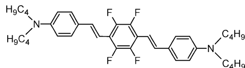
Figure 7. Molecular structure of compound 2 .
