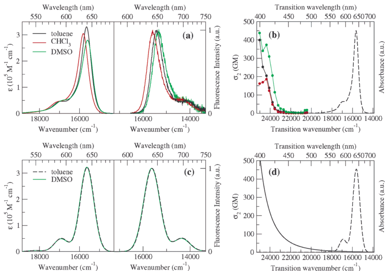
Figure 10. Spectra of compound 3. (Top panels) Experimental absorption and fluorescence (a) and TPA spectra (b) in solvents of increasing polarity (the OPA spectrum in toluene is reported for a comparison). (Bottom panels) Calculated absorption and fluorescence in two solvents of different polarity (c) and TPA spectrum in an apolar solvent (d) (the OPA spectrum is reported for a comparison). Calculated spectra have been obtained by fixing the following parameters: \eta = 0.28 eV, \sqrt{2}t = 1.20 eV, \omega_v = 0.16 eV, \epsilon_v = 0.16 eV, HWHM = 0.05 eV, and \mu_0 = 21 D. \epsilon_{or} = 0 and 0.25 eV for toluene and DMSO, respectively.
