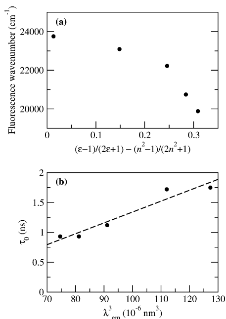
Figure 6. (a) Emission frequency of compound 1 versus the solvent polarity indicator ( \epsilon is the dielectric constant, and n is the refractive index). (b) Radiative lifetime versus \lambda_{em}^3 (●) and corresponding linear regression (---).
