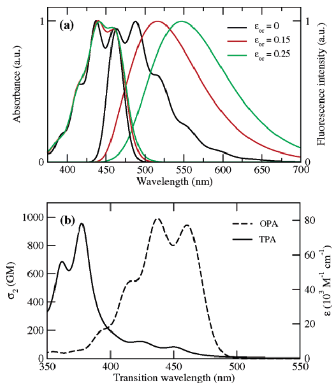
Figure 8. Calculated spectra for compound 2 . (a) Absorption and fluorescence in solvents of increasing polarity; (b) OPA and TPA in an apolar solvent. Calculated spectra have been obtained by fixing the following parameters: \eta = 1.25 eV, \sqrt{2}t = 0.80 eV, \omega_v = 0.15 eV, \epsilon_v = 0.42 eV, HWHM = 0.07 eV, and \mu_0 = 28 D. Values for \epsilon_{or} are in the legend (in electronvolts).
