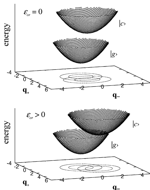
Figure 2. PES for the ground state and the OP-allowed excited state for a chromophore with \rho = 0.2 , \sqrt{2}t = 1 eV, and \epsilon_v = 0.2 eV. (Top panel) \epsilon_{or} = 0 (apolar solvent); (bottom panel) \epsilon_{or} = 1 eV (strongly dipolar solvent) and reaction field ( F_R ) fixed at its local equilibrium value for the c state.
