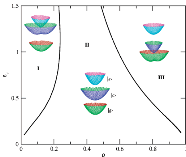
Figure 1. Phase diagram for quadrupolar chromophores, describing the stability of the different states (according to the PES sketched in each region) as a function of \rho (the quadrupolar character) and \epsilon_v (the electron-vibration coupling, in units of \sqrt{2}t ). The three PES in each region show, in order of increasing energy, the ground state (g), the OP state (c), and the TP state (e). Region I, stable ground state and bistable OP state; region II, all PES have a single minimum; and region III, the ground-state PES has a double minimum. The TP state always has a single minimum.
