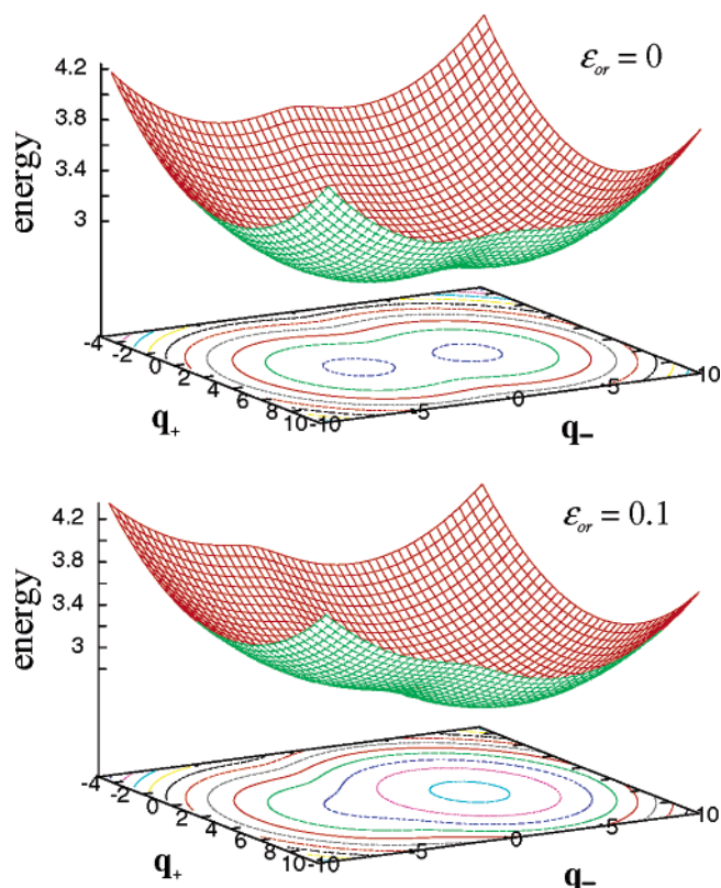
Figure 3. PES for the OP-allowed excited state for a class I chromophore with \rho = 0.07 , \sqrt{2}t = 0.6 eV, and \epsilon_v = 0.3 eV. (Top panel) \epsilon_{or} = 0 (apolar solvent); (bottom panel) \epsilon_{or} = 0.1 eV (low–medium polarity solvent) and reaction field ( F_R ) fixed at its local equilibrium value for the c state.
